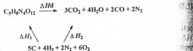
Figure 5.4 Enthalpy of detonation for PETN using Hess's law
