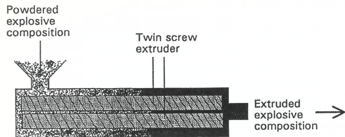
Figure 7.9 Schematic diagram of twin screw extrusion
