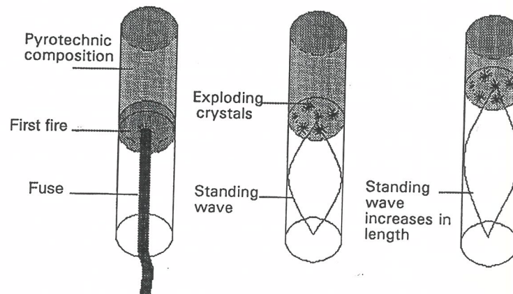
Figure 8.4 Schematic diagram of a whistling firework
