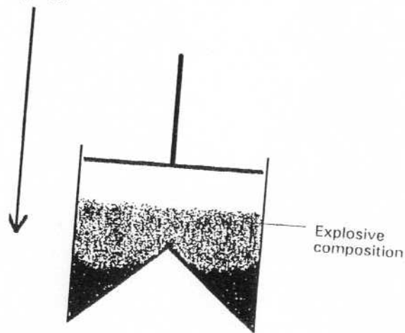
Figure 7.4 Schematic diagram of incremental pressing
