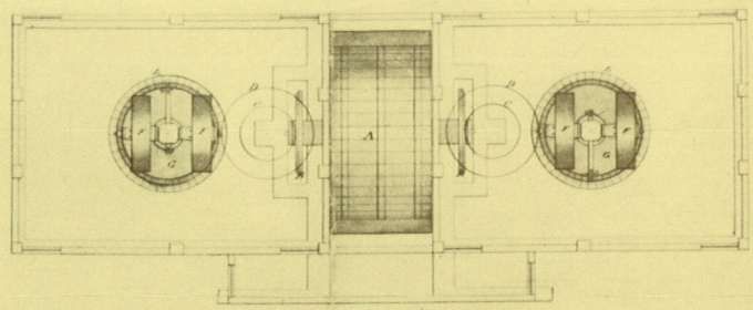
Ground Plan.
