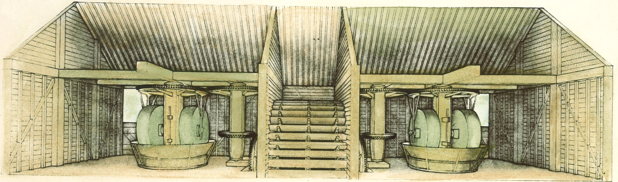
PERSPECTIVE VIEW OF THE INTERIOR.
