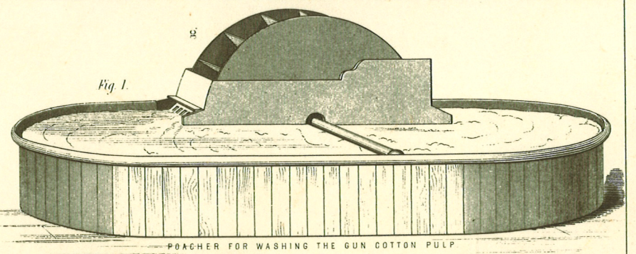
POACHER FOR WASHING THE GUN COTTON PULP.
