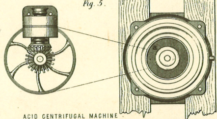
ACID CENTRIFUGAL MACHINE FOR REMOVING THE LARGE EXCESS OF ACID USED IN DIPPING PROCESS.
