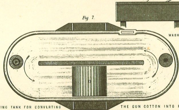
BEATING TANK FOR CONVERTING THE GUN COTTON INTO PULP.
