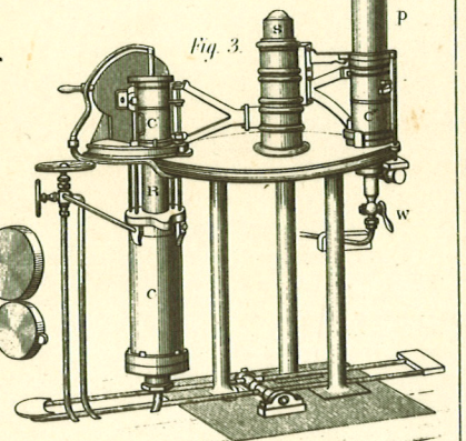
№ 2 HYDRAULIC PRESS.
