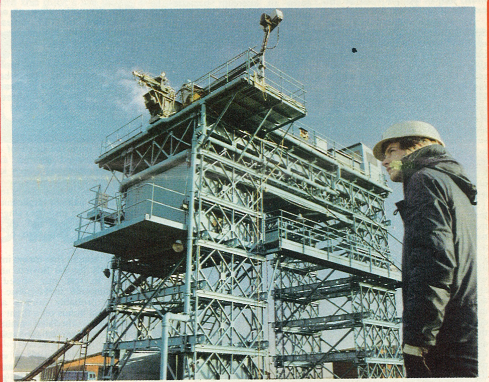
This tower at Westcott provides a mounting for certain rocket motor test firings, e.g. for measurement of exhaust plume structure.
