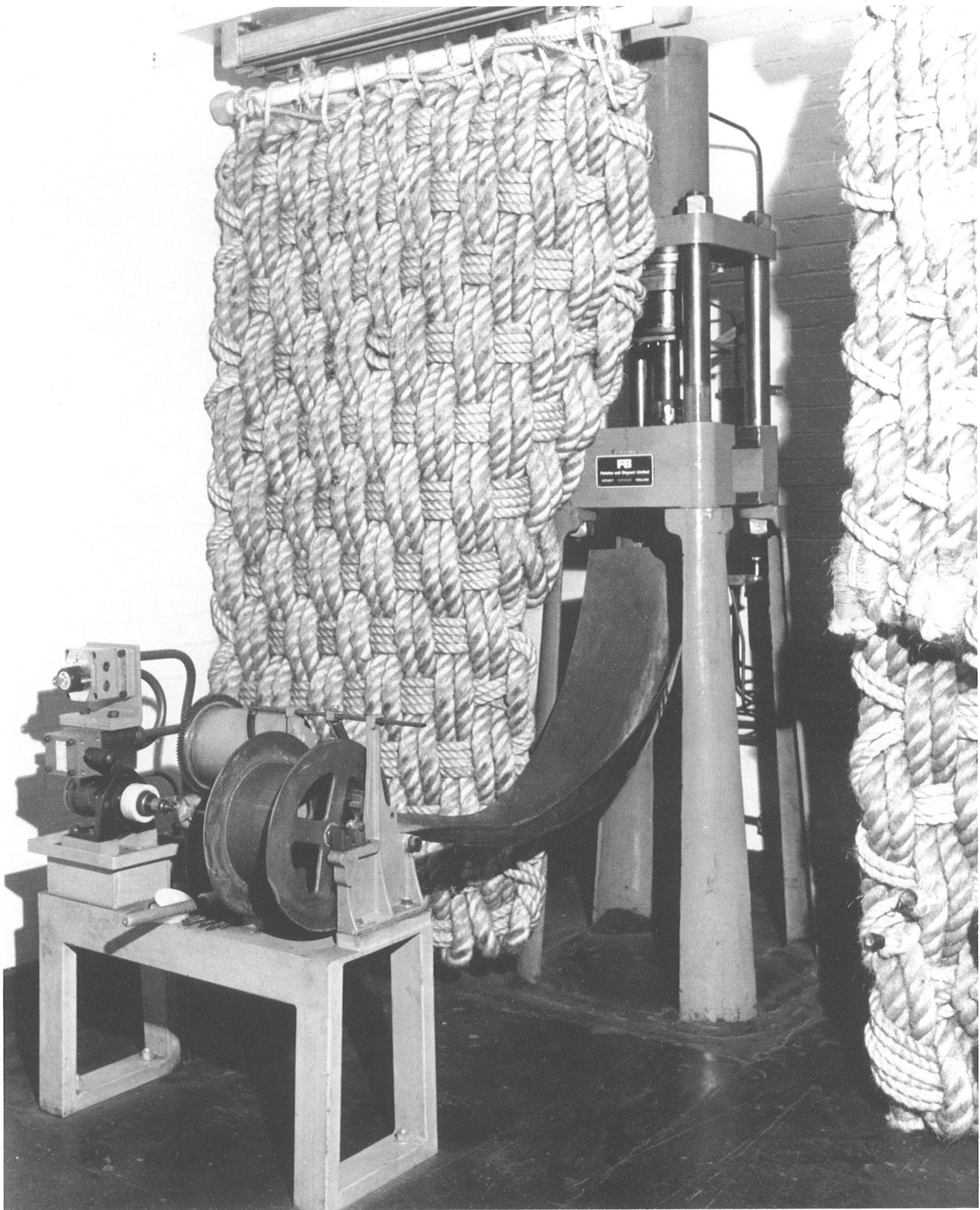
A smaller scale cordite press showing rope mantlets and guide chute
