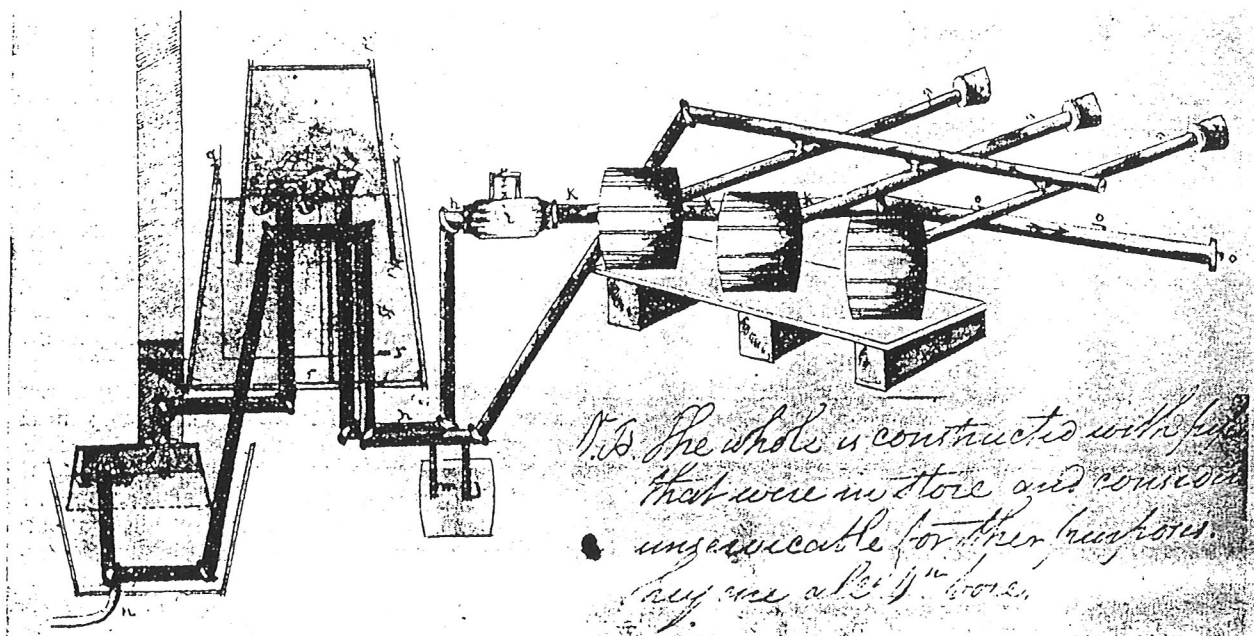
A sketch of "the gasometer" used in Congreve's research into charcoal production.
