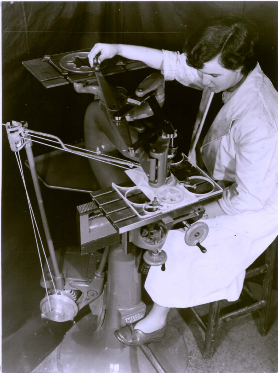
USE OF PANTOGRAPH ENGRAVING MACHINE FOR PREPARATION OF PHOTOELASTIC STRESS ANALYSIS MODELS.
