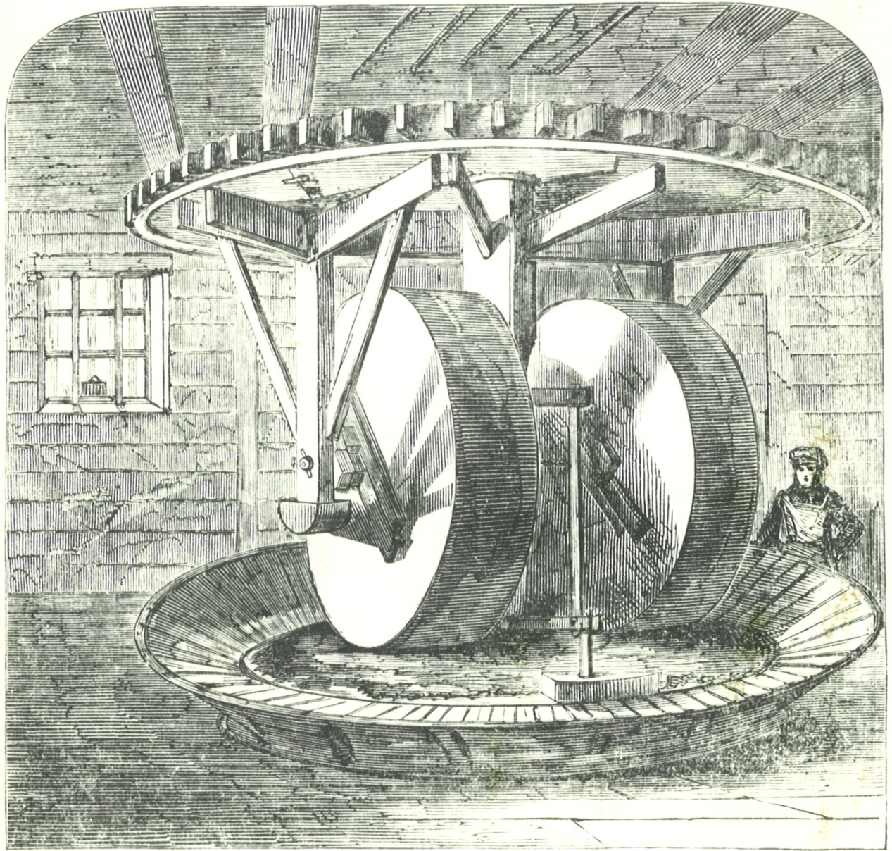
THE INCORPORATING-MILL.
